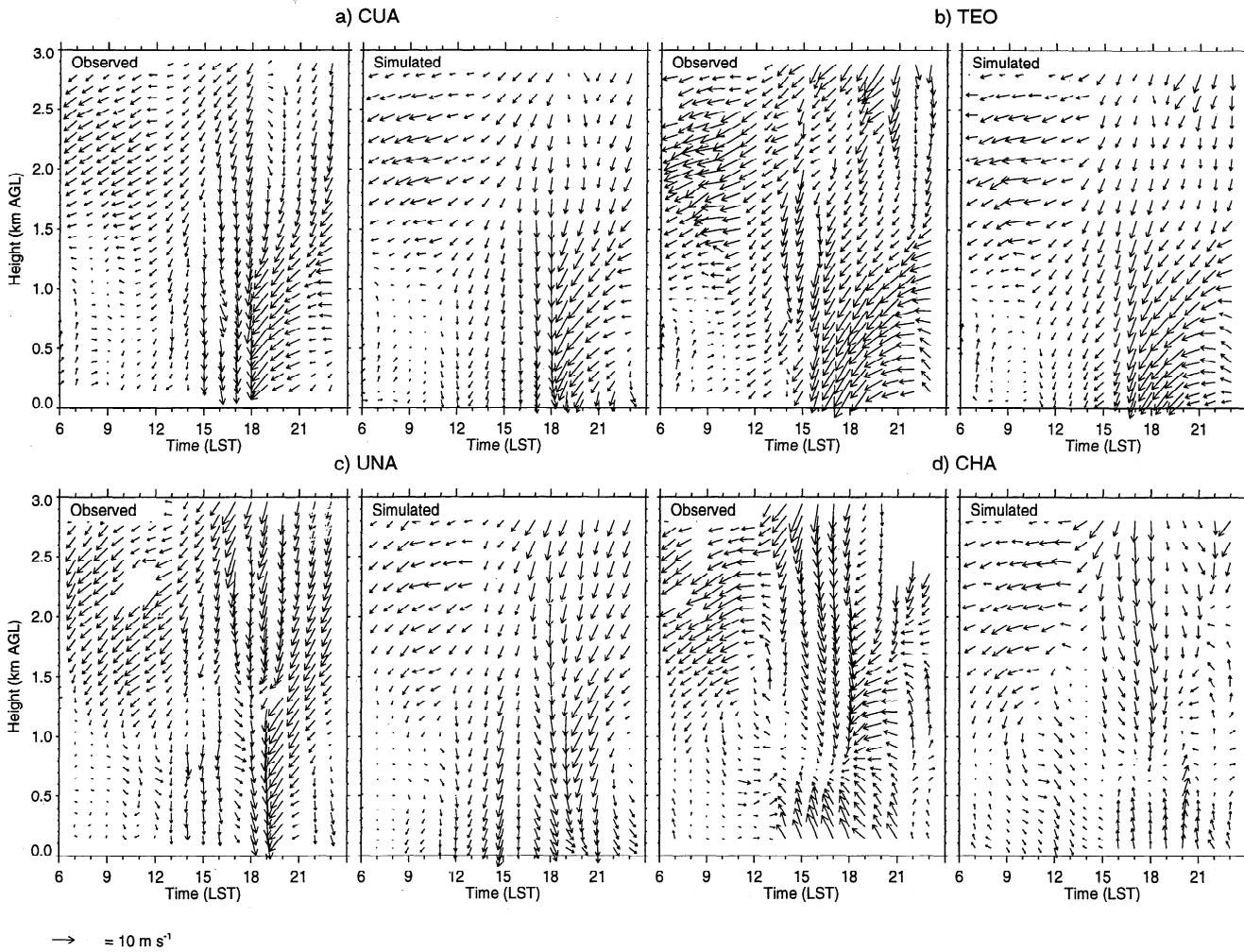
Figure 13. Simulated and observed hourly horizontal wind vector profiles on March 4, 1997, at (a) Cuautitlan, (b) Teotihuacan, (c) UNAM, and (d) Chalco.
