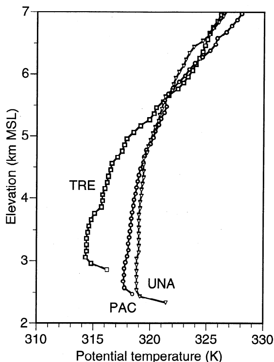
Figure 4. Mean potential temperature soundings at 1630 LST at UNAM, Pachuca, and Tres Marias. Soundings are averaged from all available soundings (12 at TRE, 20 at PAC, and 22 at UNA) at the 1630 observation time during the February 23 to March 22, 1997, experimental period.
