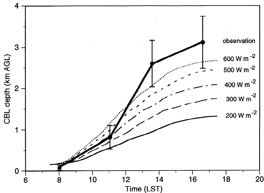
Figure 3. Mean (dots) and standard deviations (error bars) of observed convective boundary layer (CBL) depths at Teotihuacan. Also shown are CBL depths estimated with a simple encroachment model given sinusoidal surface sensible heat fluxes with the indicated amplitudes using the mean 0800 LST sounding as an initial condition.
