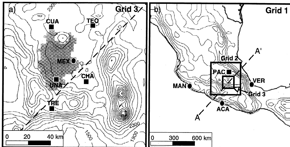
Figure 1. Topography of Mexico. (a) Map of the Mexico Basin, showing the locations of the Investigation sobre Materia Particulada y Deterioro Atmosferico-Aerosol and Visibility Research (IMADA-AVER) radar profiler/ radiosonde sites (squares), the Mexico City airport rawinsonde site (dot), and the Mexico City metropolitan area (shaded). The topographic contour interval is 200 m. (b) Three coastal Mexican rawinsonde sites (dots), a GPS rawinsonde site (square), the three nested Regional Atmospheric Modeling System (RAMS) simulation grids, and the cross-section A-A' through the isthmus used in two-dimensional model simulations. The topographic contour interval is 500 m. Site abbreviations are as follows: ACA, Acapulco; CHA, Chalco; CUA, Cuautitlan; MAN, Manzanillo; MEX, Mexico City International Airport; PAC, Pachuca; TEO, Teotihuacan; TRM, Tres Marias; UNA, UNAM; VER, Veracruz.
